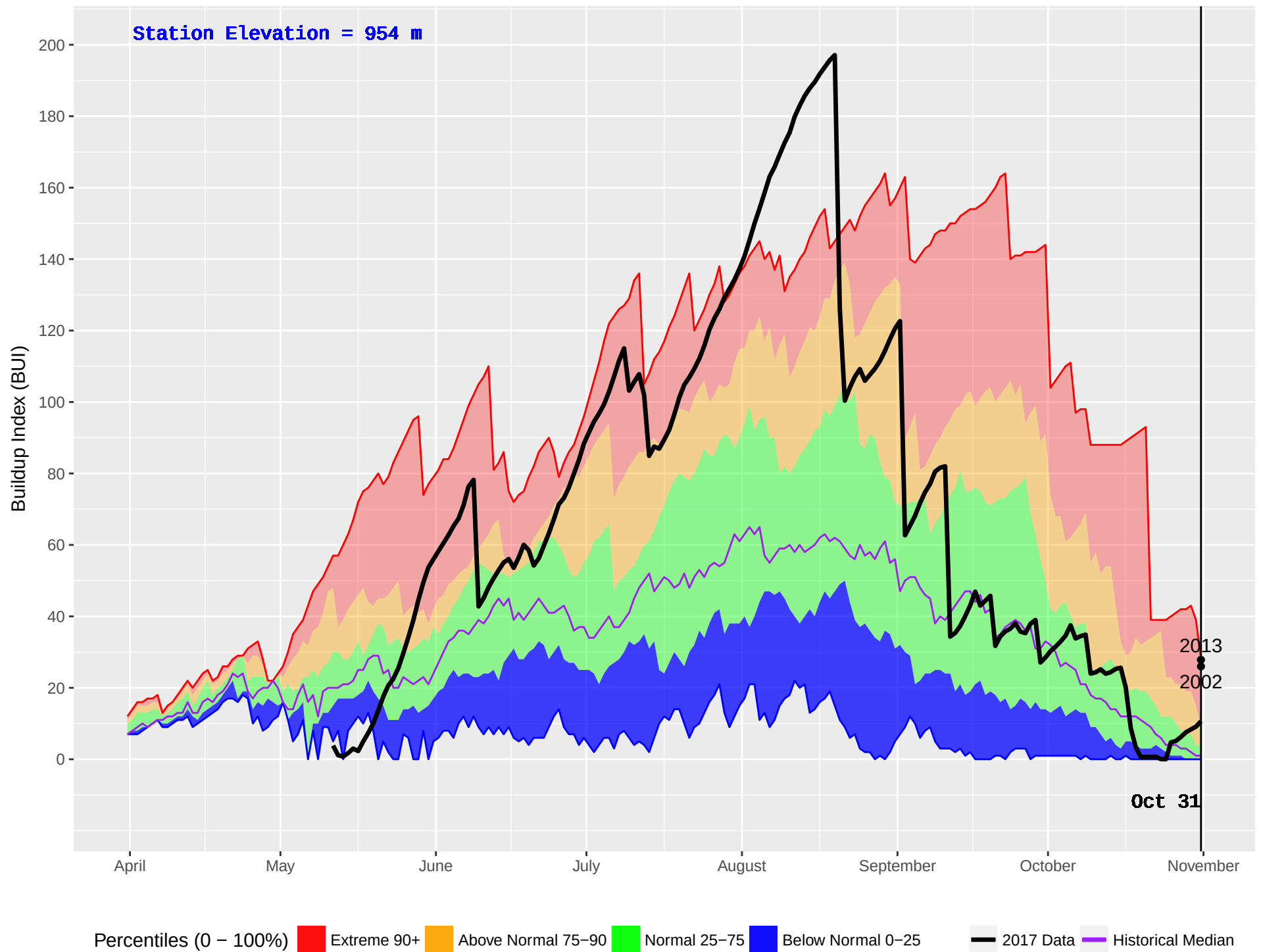
NADINA (179) : Historical (1985–2016) and Current (2017) Noon Buildup Index (BUI)
